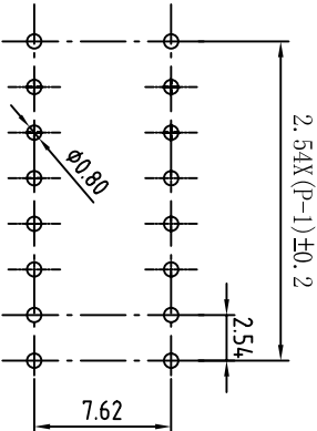
[P.C.B LAYOUT]
