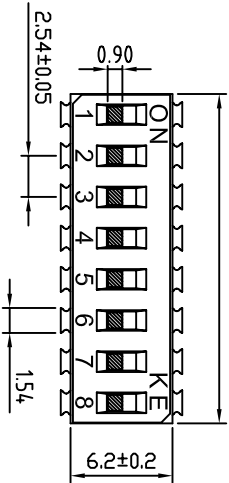
[Dimensions] (A)
