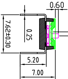
[推钮行程]
