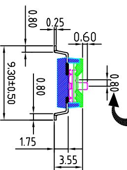
[推钮行程]
